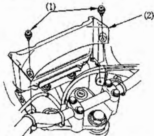
(1) Circlips
